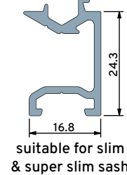
New & Improved Sash Extension
