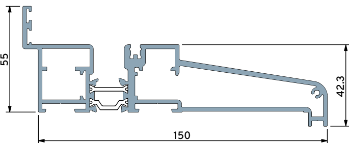
Integrated Outerframe 150mm Cill with Screwports
