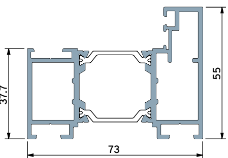
Slim Sash (55mm) (for doors up to 3000mm high)
