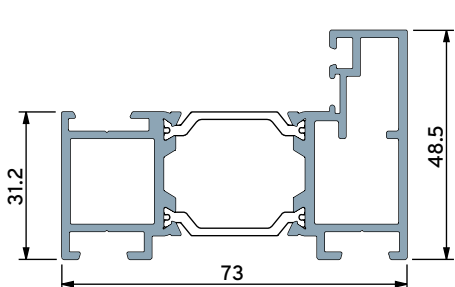
Ultra Slim Sash (48.5mm) (for doors up to 2600mm high)
