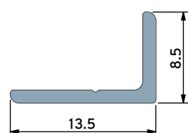
BF73 / WF73 Connecting Profile
