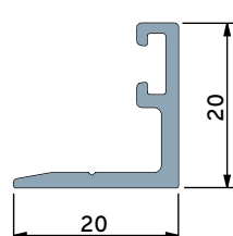
Low Threshold Rebate Add-On
