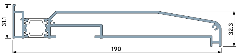
190mm Cill with Screwports
