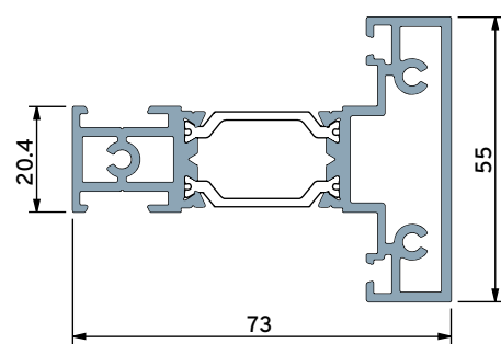
Transom for Sash
