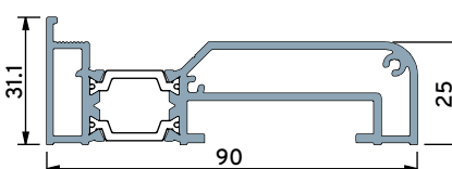
90mm Stub Cill with Screwports
