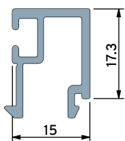
Glazing Bead for 32mm DGU
