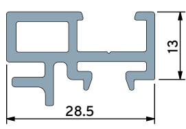
Super Slim Keep Adaptor
