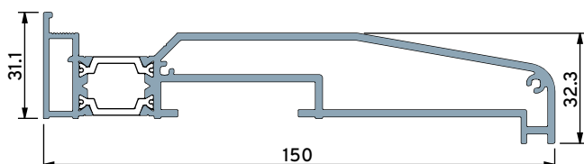
150mm Cill with Screwports
