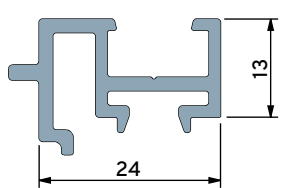
Super Slim Lock Adaptor
