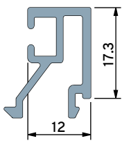
Glazing Bead for 36mm DGU
