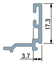
Glazing Bead for 44mm DGU
