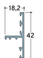
TV 8003 6,0m 340 gr/m Frame Rain Cover
