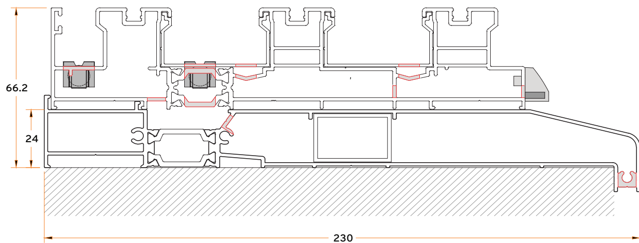
TH 8022 Sub Cill 230mm & Drainage
