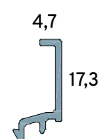
TV 80503 6,0m 133gr/m Clip for Glass Sash
