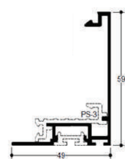
PP-80306 Plastic Spacer for 50mm Interlock (TH 80411)
