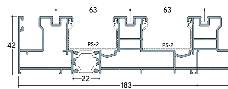
TH 8022 6,5m 3.093 gr/m Triple Rail (Successive)
