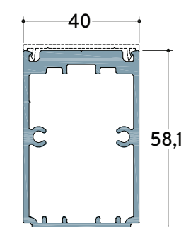
TV 00628 6,5m 1.489 gr/m Reinforcement Profile New Profile for Interlock 50mm
