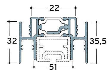
TH 8045 6,0m 1.777 gr/m Adjoining profile for Glass Sash
