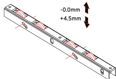
RO-80701 Quadrable Roller for Glass Sash
