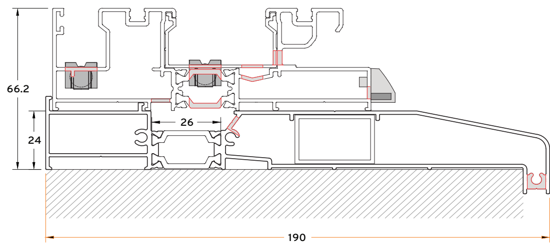
TH 80113 Sub Cill 190mm & Drainage
