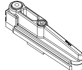
PS-002020 Dampening Stopper for Glass Sash
