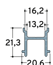
TV 8011 6,0m 279 gr/m Sash Spacer for Lock
