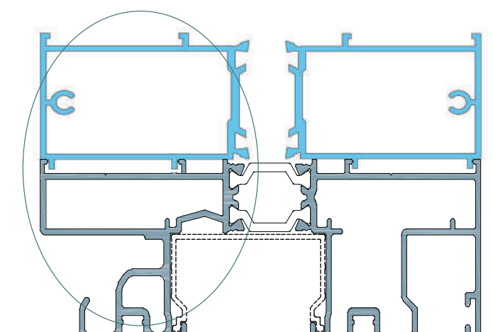
NT-80616 Detail 1 per either side of frame TH80113 or TH8022
