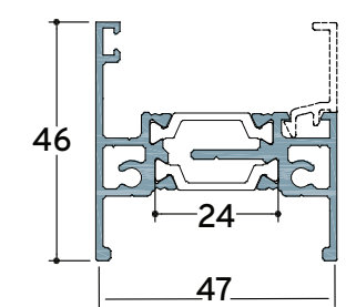
TH 80411 6,5m 1.027 gr/m Interlock Profile 50mm with Clip New Profile for Interlock 50mm
