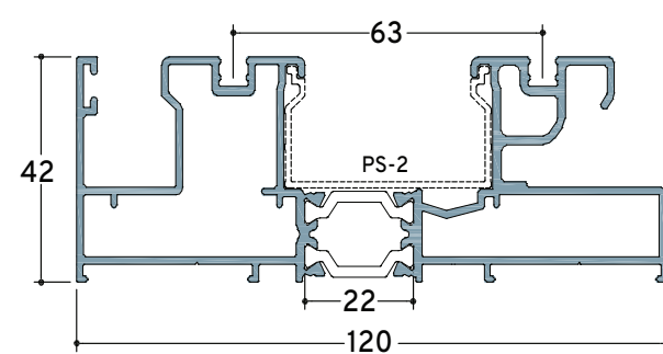
TH 80113 6,5m 2.157 gr/m Double Rail (Successive)
