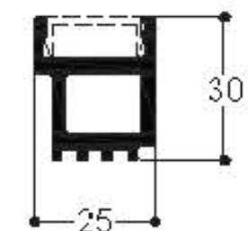
TV 00627 Reinforcement Grip
