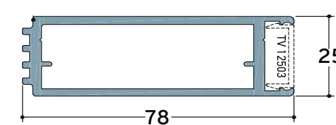
TV 12603 6,5m 1.368 gr/m Reinforcement Profile for 25mm Interlock
