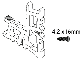
PS-10 Corner Joint for TH 8040
